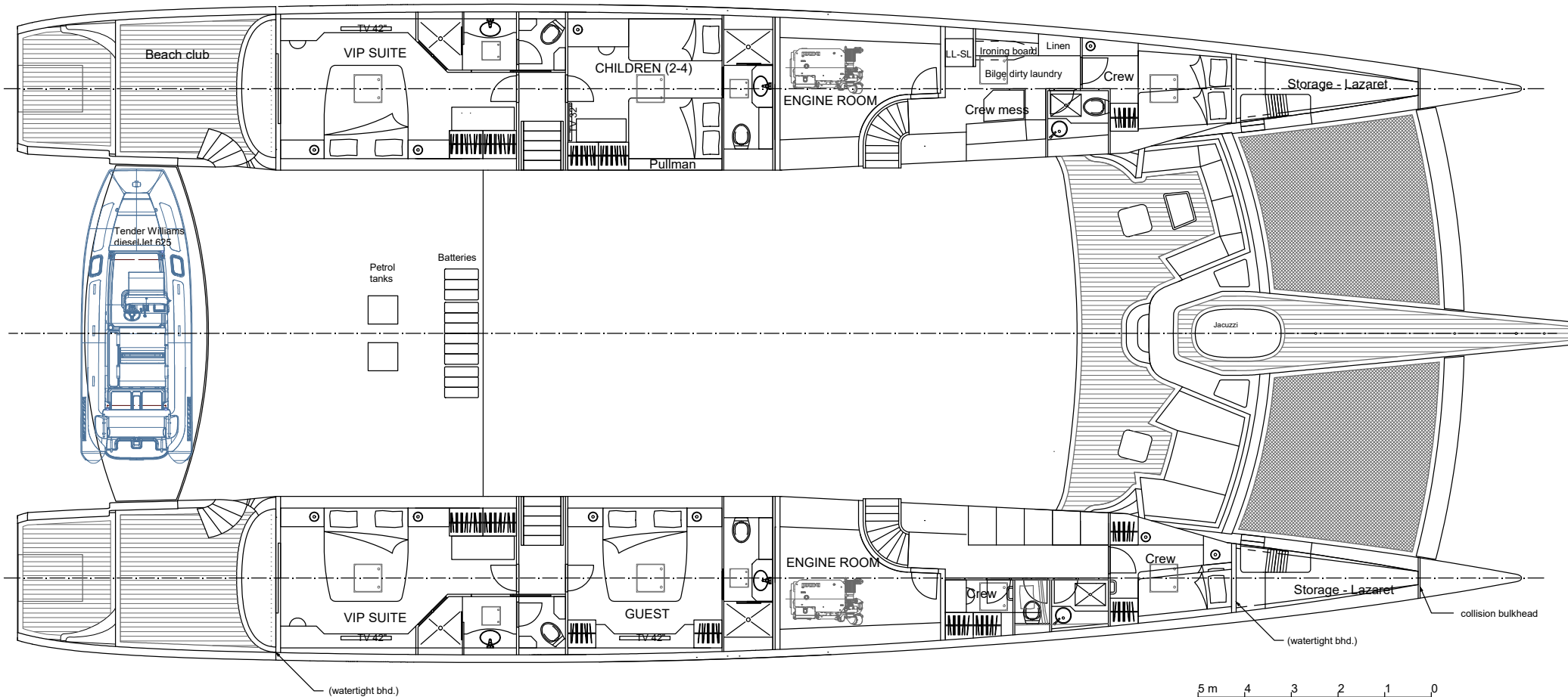
Plan view - Lower deck
