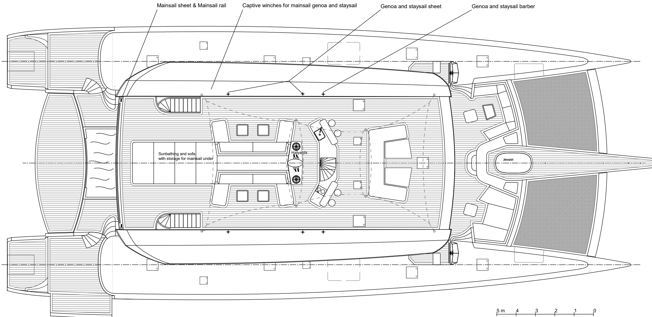
Plan view - Fly bridge
